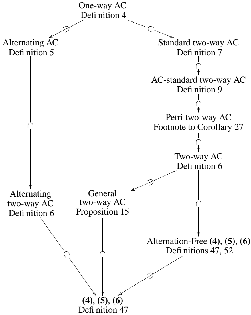
Fig. 1. AC-tree automata considered in this paper
