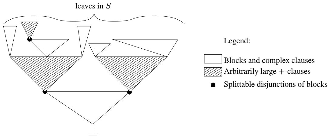
Fig. 3. Grey zones, fat dots, white zones
